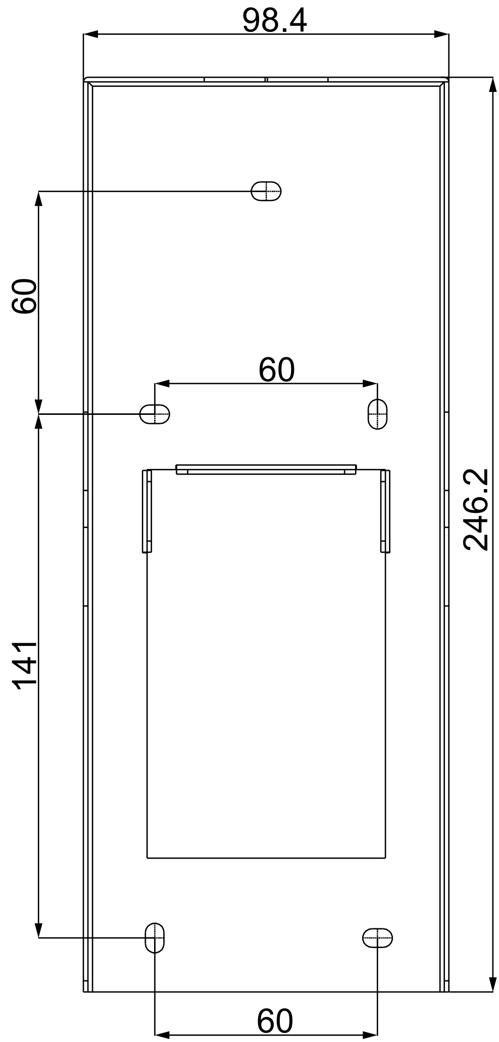
1 FRONT VIEW
