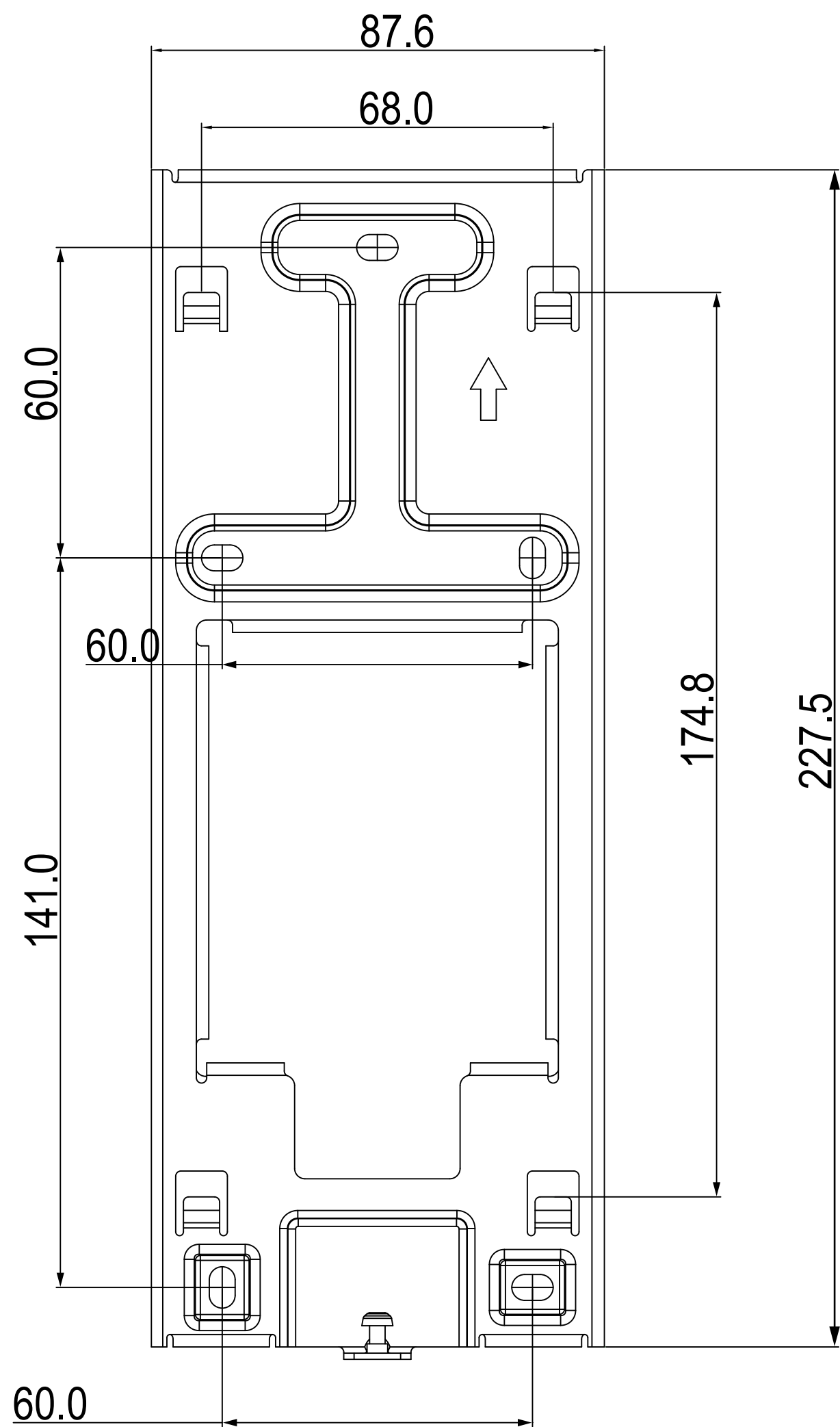
1 FRONT VIEW
